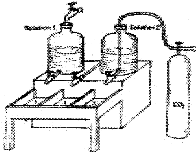
Deacidification with calcium hydroxide and calcium bicarbonate
